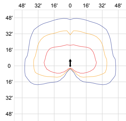
16' Lens Height, High Output, Clear Lens, Type IV
