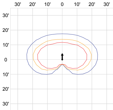
10' Lens Height, Low Output, Frosted Lens, Type II
