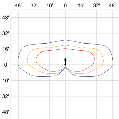
16' Lens Height, High Output, Clear Lens, Type II
