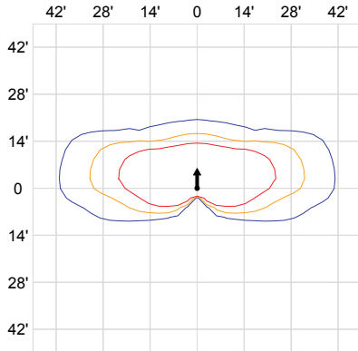
14' Lens Height, Low Output, Clear Lens, Type II
