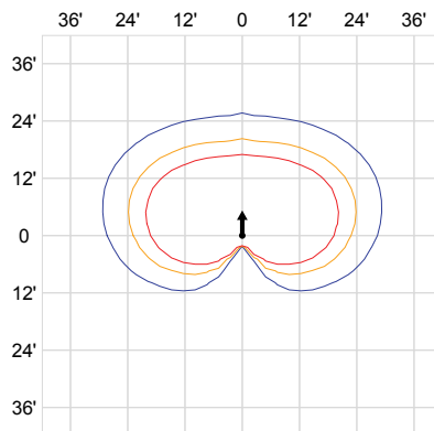
12' Lens Height, High Output, Frosted Lens, Type III
