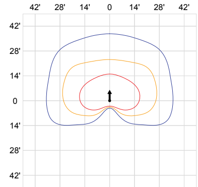
14' Lens Height, Low Output, Clear Lens, Type IV
