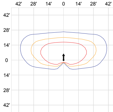
14' Lens Height, Low Output, Clear Lens, Type III
