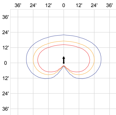
12' Lens Height, High Output, Frosted Lens, Type II
