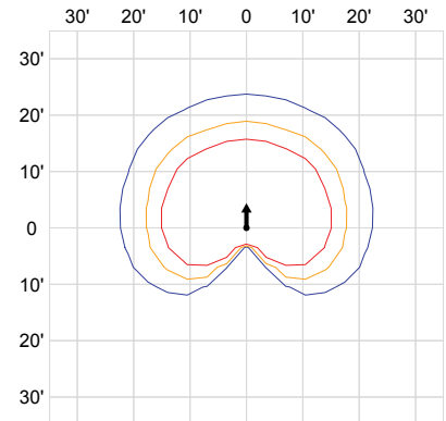
10' Lens Height, Low Output, Frosted Lens, Type IV
