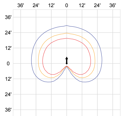
12' Lens Height, High Output, Frosted Lens, Type IV
