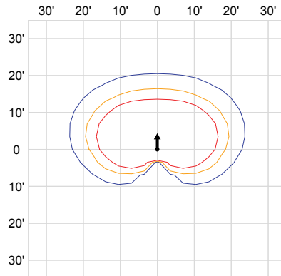
10' Lens Height, Low Output, Frosted Lens, Type III
