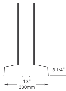
Base Cover
