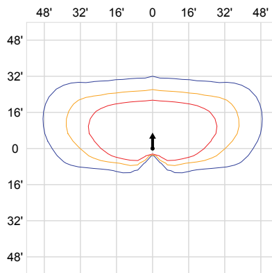
16' Lens Height, High Output, Clear Lens, Type III
