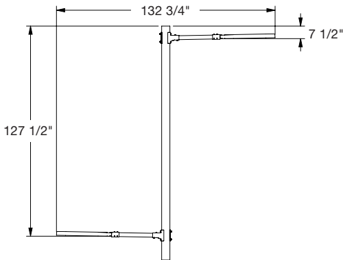
30-C CLB-SS-30 Weight: 63 lbs
