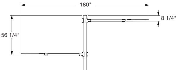
20-C CLB-SS-53 Weight: 71.4 lbs
