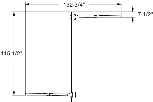
25-C CLB-SS-30 Weight: 63 lbs
