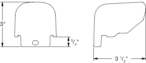
Aluminum Pole Nut Covers
