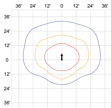
12' Lens Height, Type IV
