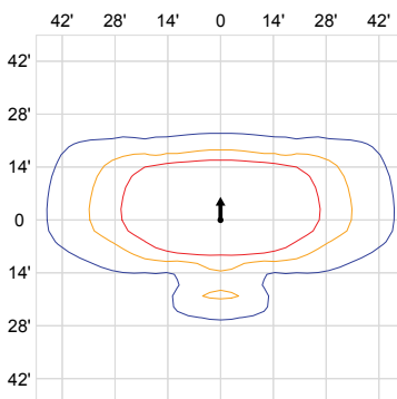
14' Lens Height, Type II
