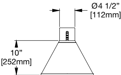
DZ401 Weight without Louvre: 21 lbs Weight with Louvre: 22.7 lbs EPA: 0.3954ft 2
