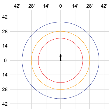
14' Lens Height, Type V
