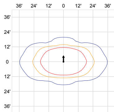
12' Lens Height, Type I
