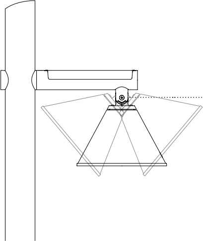
Tilt adjustable luminaire for accent lighting Up to 50° tilt in 10° increments.
