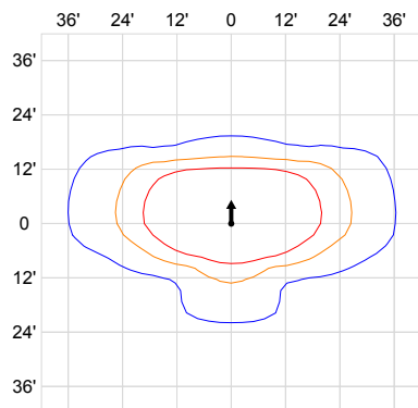
12' Lens Height, Type II
