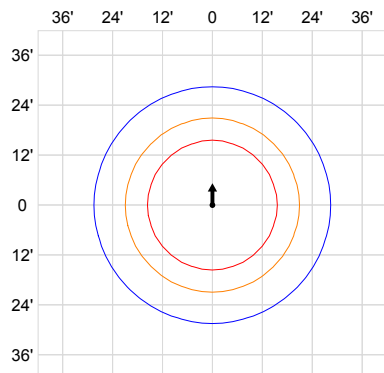
12' Lens Height, Type V
